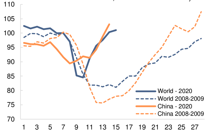
Merchandise exports in volume (100 = Sept. 2008 and 100 = Feb 2020 for world, Dec 2019 for China)
